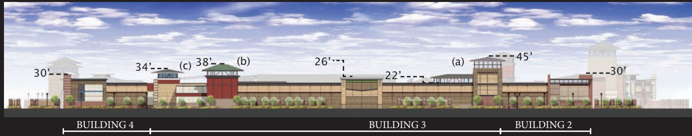
REVISED SOUTH ELEVATION
