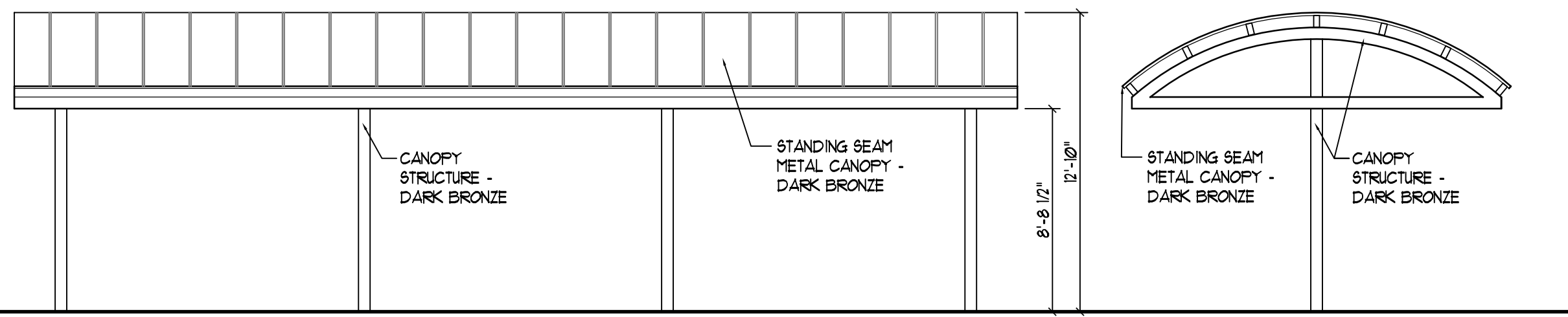
PAY STATION CANOPY ELEVATIONS SCALE: 3/16" = 1'-0"
