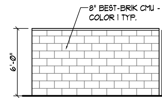
TRASH ENCLOSURE ELEVATIONS SCALE: 3/16" = 1'-0" (23'-4" X 11'-4" ENCLOSURE)
