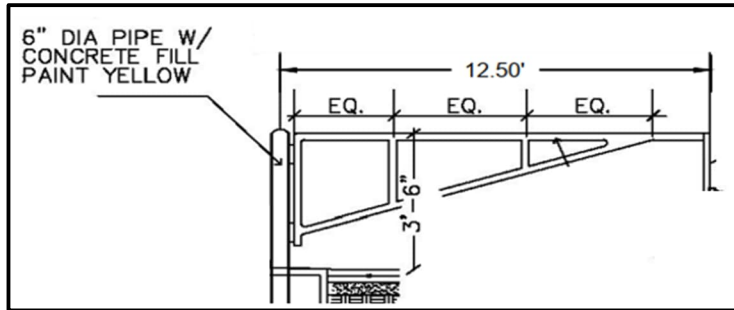
Figure 4: Proposed swing gate
