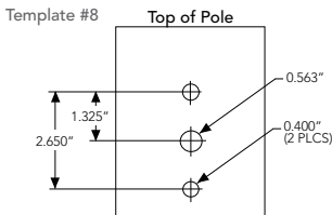
Handhole
