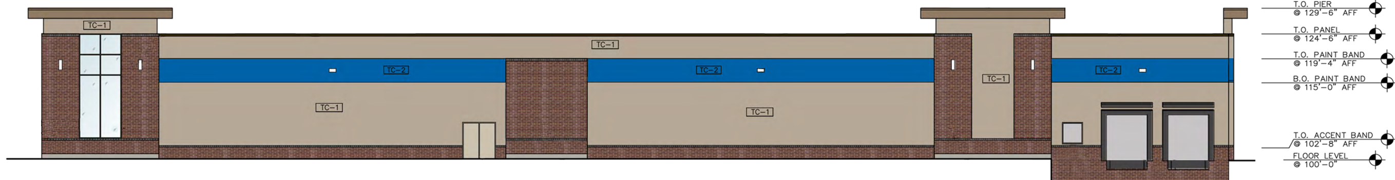
2 SIDE ELEVATION 3/32" = 1'-0"
