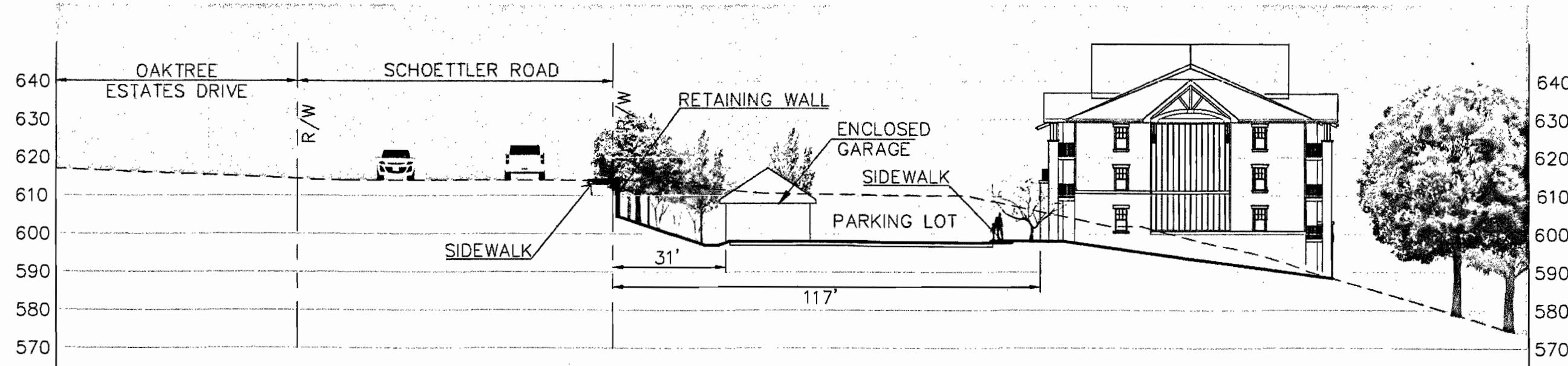
SECTION H-H SCALE 1"=30'-0"
