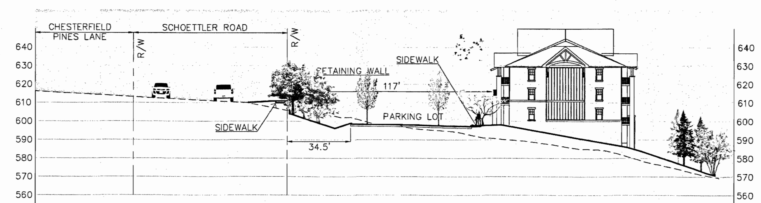
SECTION F-F SCALE 1"=30'-0"
