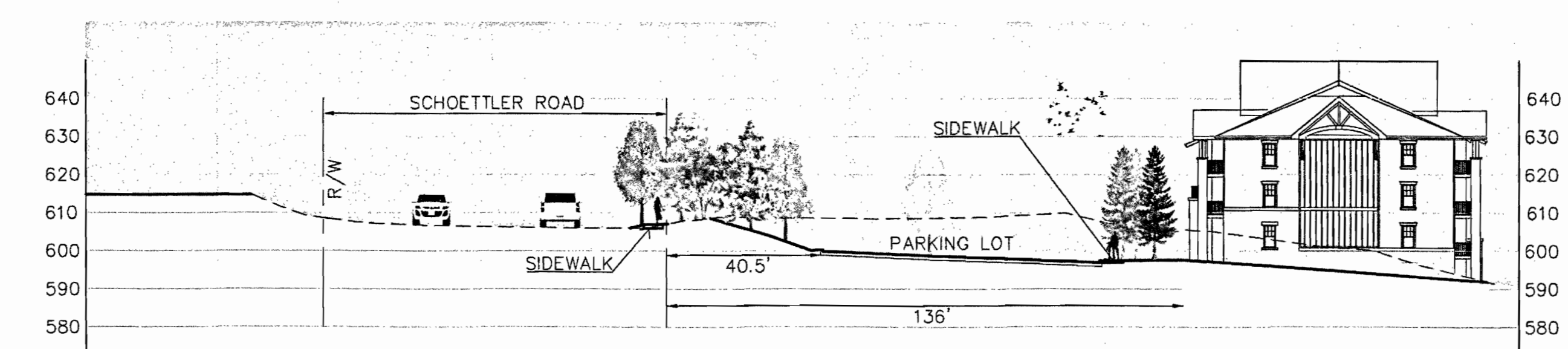
SECTION 1-1 SCALE 1"=30'-0"
