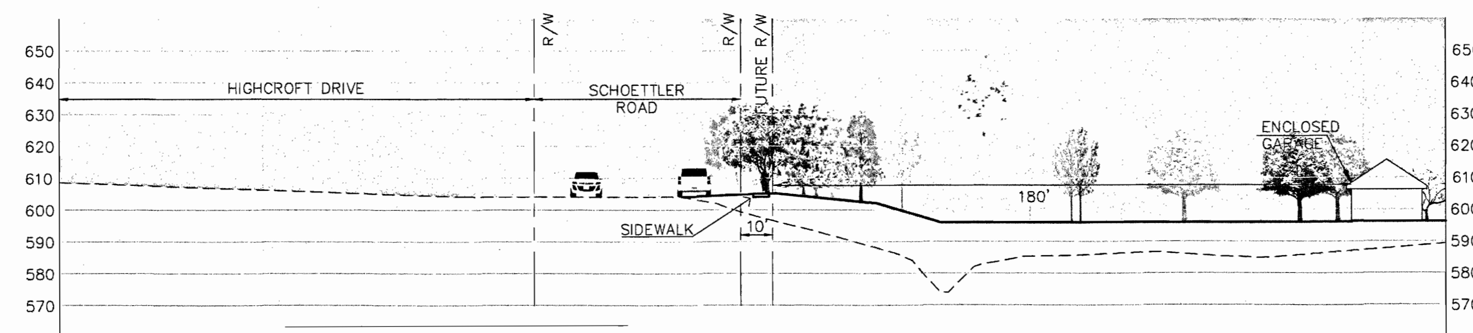
SECTION D-D SCALE 1"=30'-0"
