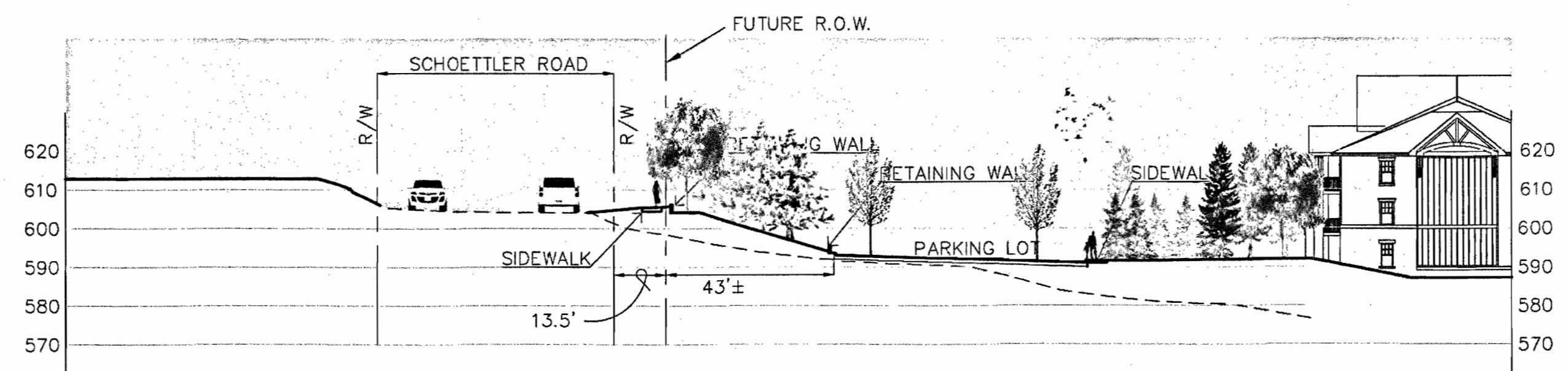
SECTION E-E SCALE 1"=30'-0"
