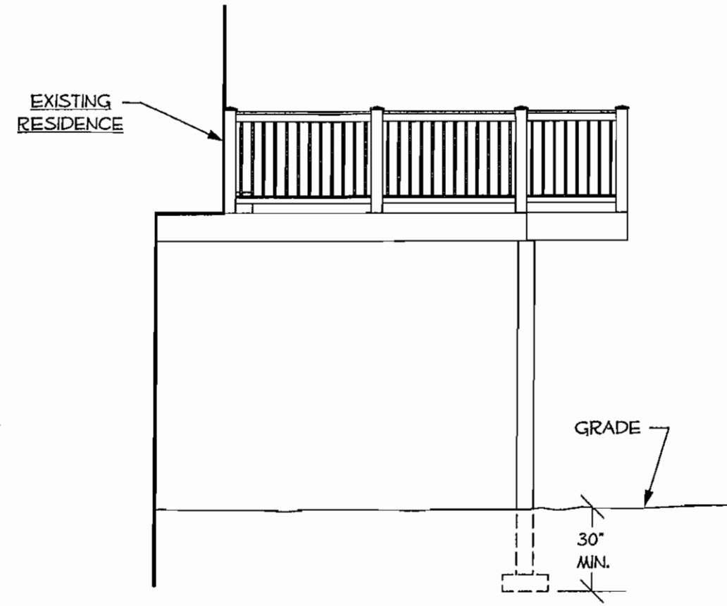
EAST ELEVATION (LOOKING WEST)
