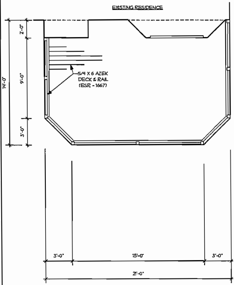
DECK - PLAN VIEW
