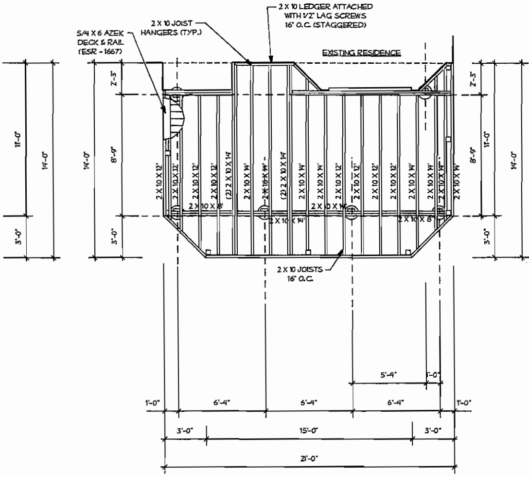
PIER, POST, BEAM & FRAMING LAYOUT
