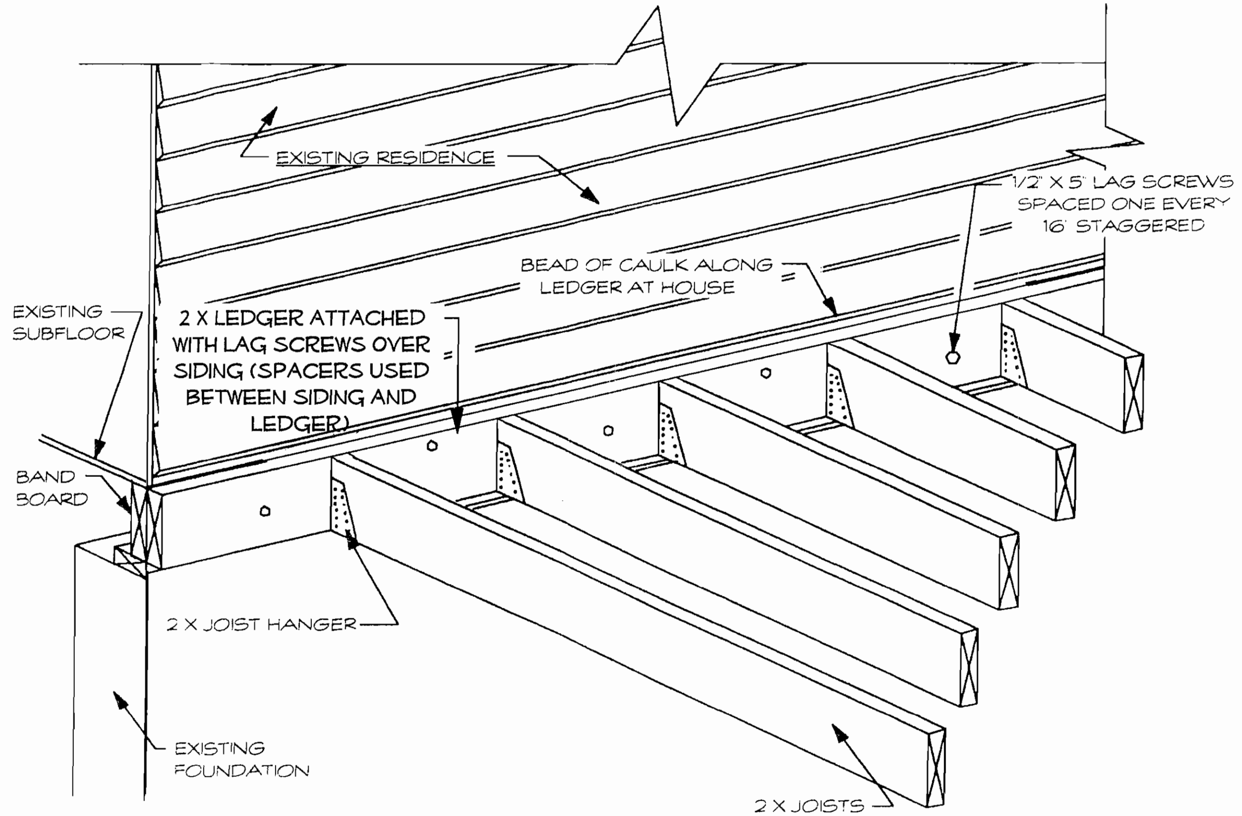
LEDGER ATTACHMENT CONSTRUCTION VIEW
