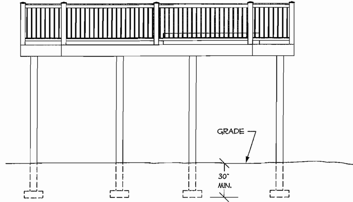
NORTH ELEVATION (LOOKING SOUTH)
