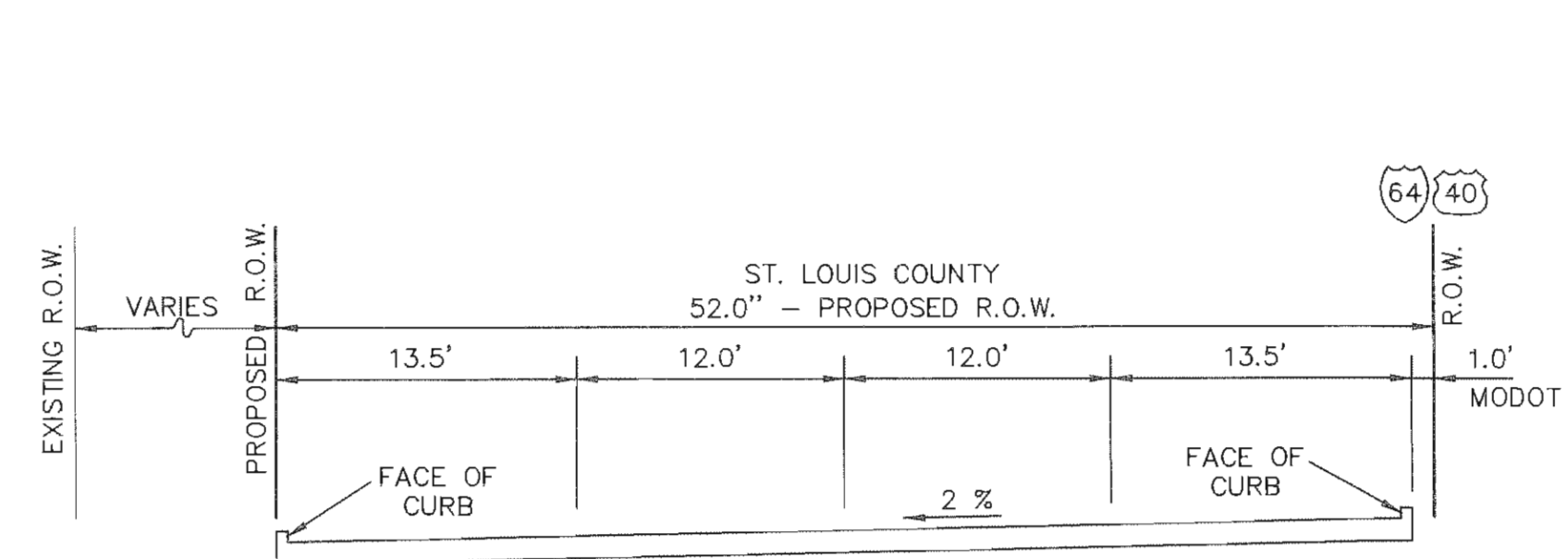
NORTH OUTER FORTY TYPICAL 4-LANE SECTION SCALE: 1"=40' NOTE: TO BE CONFIRMED BY MODOT AND/OR ST. LOUIS COUNTY
