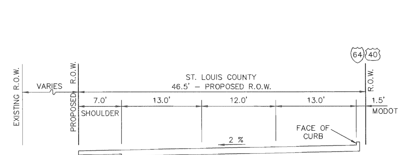
NORTH OUTER FORTY TYPICAL 3-LANE SECTION SCALE: 1"=40' NOTE: TO BE CONFIRMED BY MODOT AND/OR ST. LOUIS COUNTY
