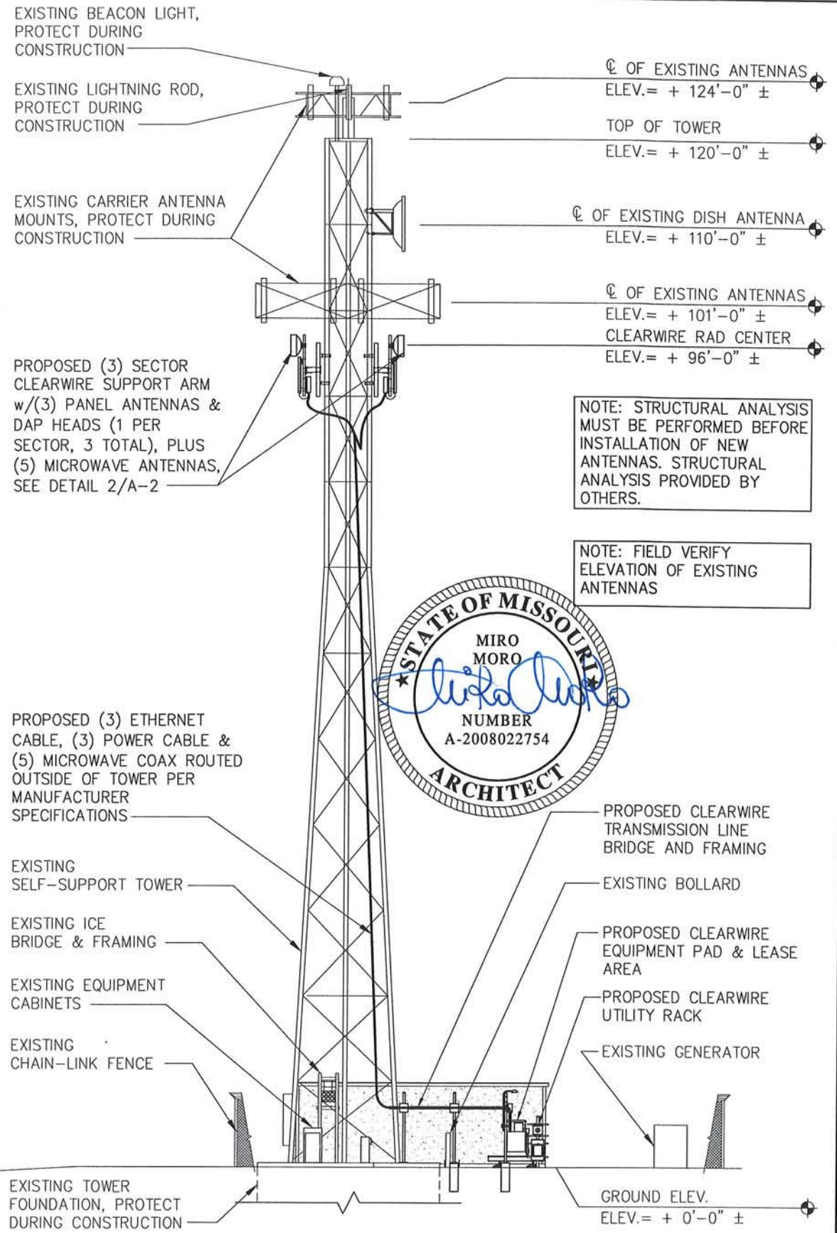
2 NORTHEAST ELEVATION (LOOKING SOUTHWEST) 11x17 SCALE: 1/16"=1'-0"
