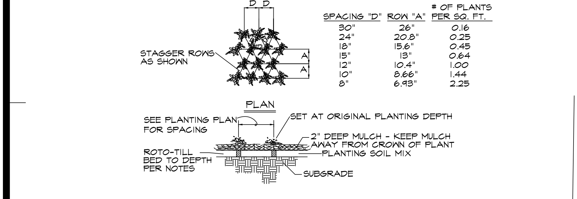
FORB/GRASS PLANTING DETAIL N.T.S.
